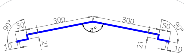
Shaped Profile 53
