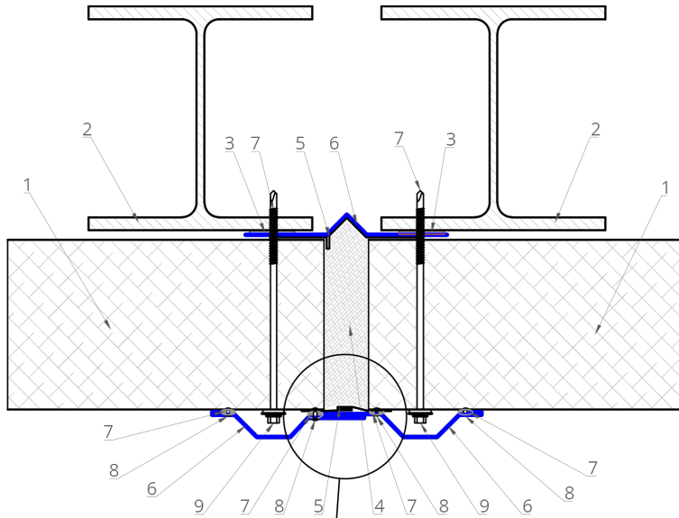
Construction node A 3:1 scale
