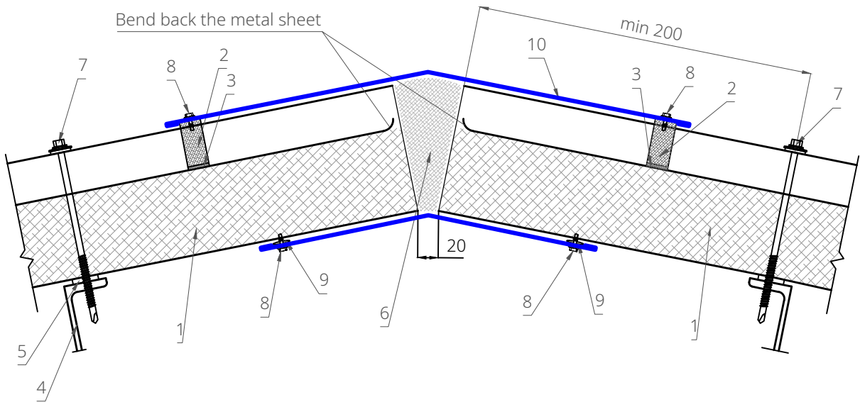
Shaped Profile 19
