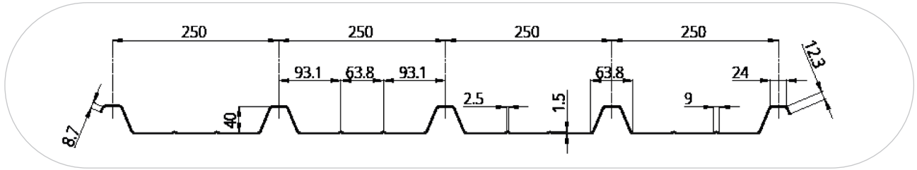
Diagram 10. Profile of the exterior surface of roofing sandwich panels (PRT Z)
