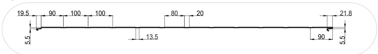
Trapezoid at increments 100 (T1)
