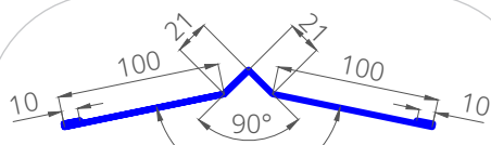
Shaped Profile 28
