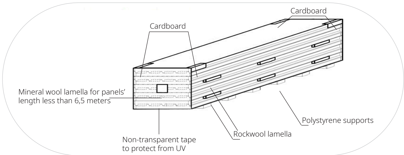
Diagram 13. Roof Sandwich Panels Packs
