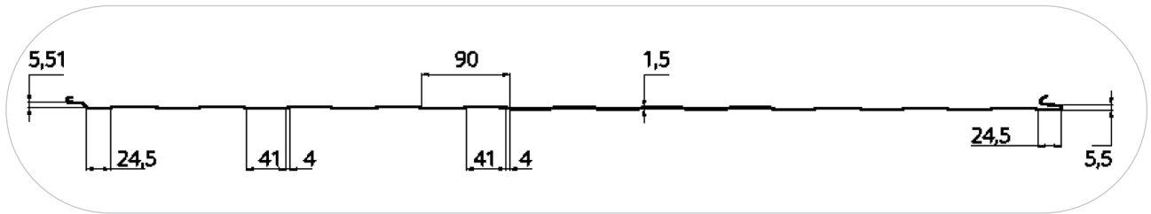
Diagram 11. Profiles of inner surface of roofing sandwich panels (PRT Z)
