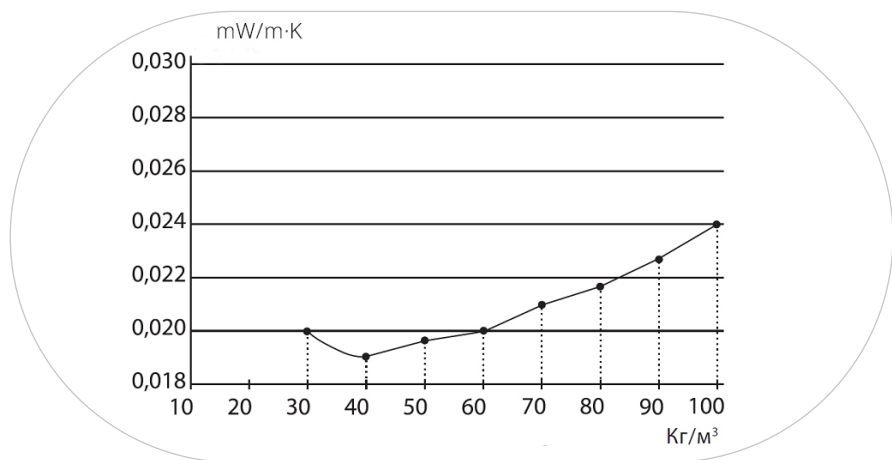
Figure 5. Relationship between thermal conductivity and density in PU foams
