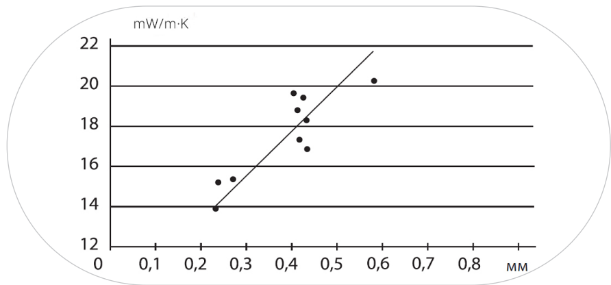
Figure 4. Relationship between thermal conductivity and average cell size in PU foams
