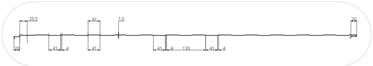
Figure 14. Types of profiles on the internal face of PWT panels
