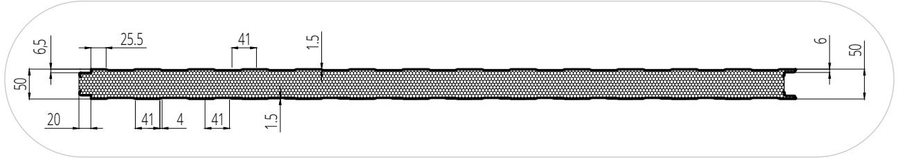
Figure 12. Geometry of wall panels with standard locking system (PWT)
