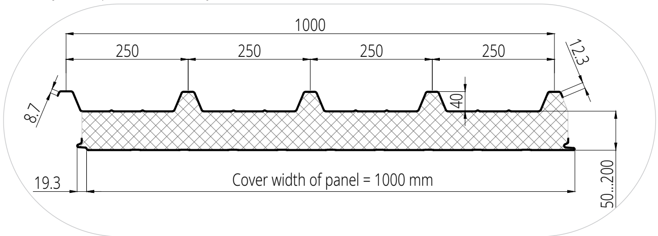
Figure 28. Geometry of roof panel with Z-Lock system (PRT Z)
