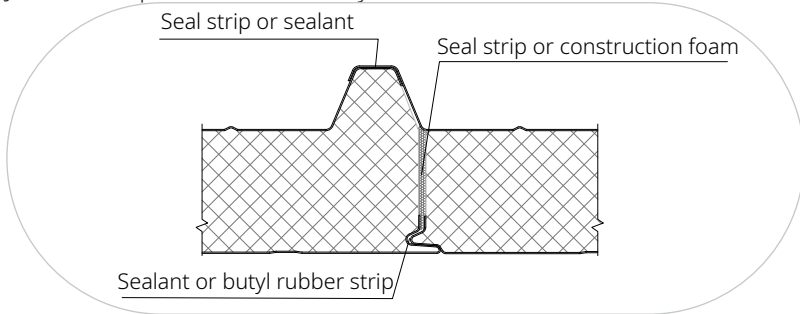
Figure 30. Types of profiles on the internal face of PRT Z panels
