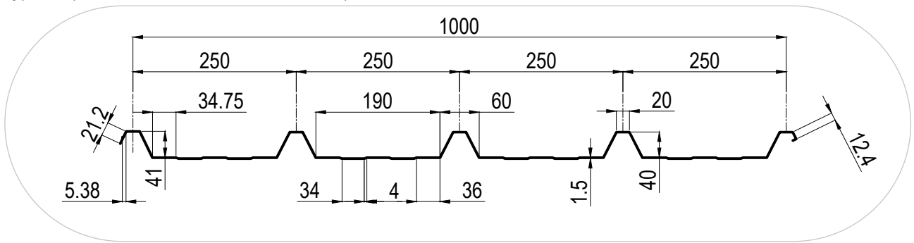
Figure 28. Geometry of roof panel with Z-Lock system (PRT Z)
