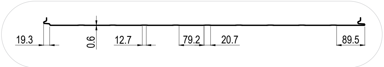
Trapezoidal profiles with 100 mm span (T1)
